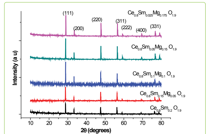
Figure 1: X-ray diffraction pattern of Ce_{0.8}Sm_{0.2-x}Mg_xO_{2-\delta} ( x = 0.00; 0.05; 0.1; 0.15, 0.175 ) sintered at 1300°C.
