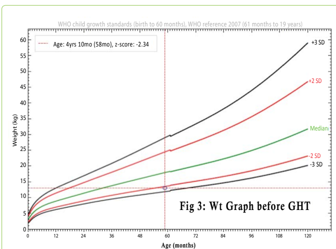
Figure 3: Weight graph with weight on -2.09 SD.
